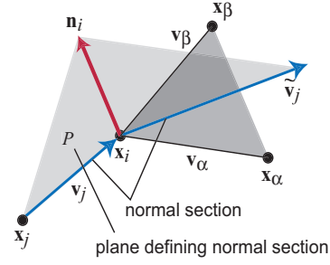
Figure 4: Computing directional derivatives using normal sections.
